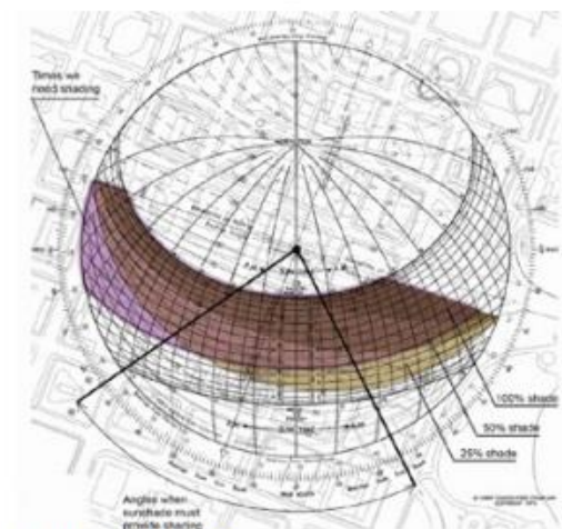
SITE STUDY 1. SOLAR ANALYSIS OF BUILDING SITE
