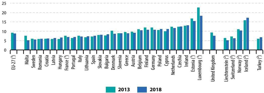
Figure 13.2: Greenhouse gas emissions per capita, by country, 2013 and 2018 (tonnes per capita)
