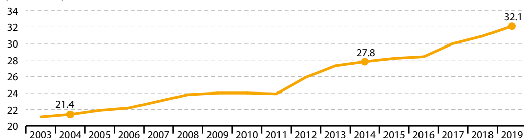
Figure 5.9: Seats held by women in national parliaments, EU-27, 2003–2019
