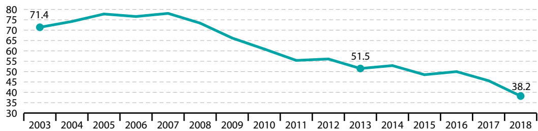
Figure 14.7: Assessed fish stocks exceeding fishing mortality at maximum sustainable yield ( F_{MSY} ) in the North-East Atlantic, 2003–2018
