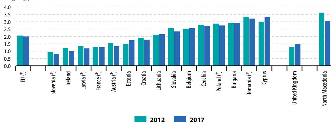
Figure 6.5: Biochemical oxygen demand in rivers, by country, 2012 and 2017
