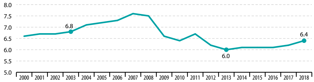
Figure 12.4: Domestic material consumption, EU-27, 2000-2018 (billion tonnes)
