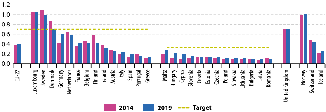
Figure 17.2: Official development assistance as share of gross national income, by country, 2014 and 2019
