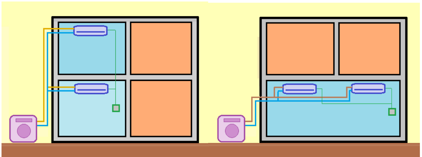
Obr. 2.17 Split systém Twin
